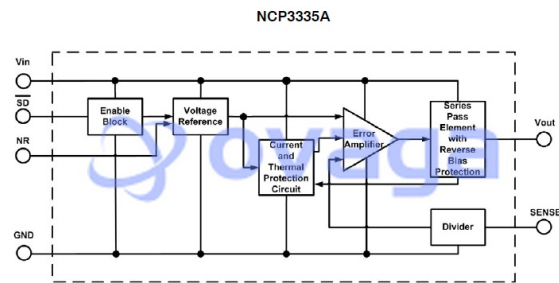
Figure 3. Block Diagram, Fixed Output Version
