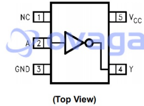
Pin Assignments for SC70
