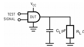
FIGURE 1. AC Test Circuit
